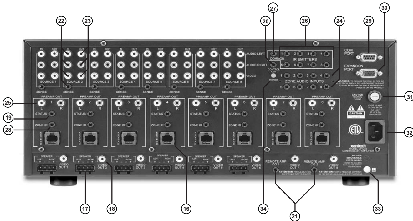
Figure 3 – The Model MRC88m Controller/Amplifier – Rear Panel Connections and Functions
