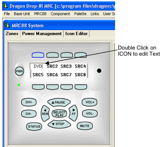
Figure 25 Entering Text Directly
