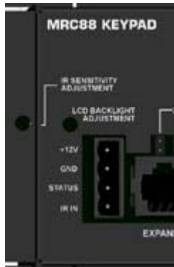
Figure 12: MRC88m Connecting Block located on rear of Keypad
