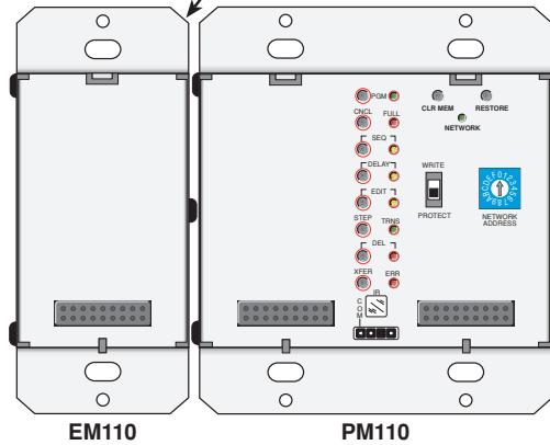
Fig. 3 EM110/PM110 Mounting Precautions
