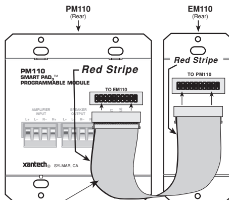
Fig. 2 3-Gang EM110 to PM110 Connections
