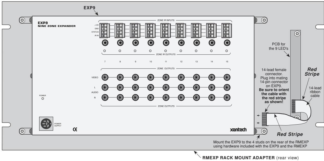
Fig. 2 The RMEXP with an EXP9 Mounted to Rear Surface
