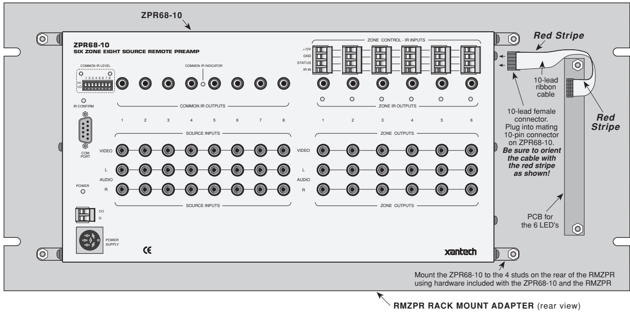
Fig. 2 The RMZPR with a ZPR68-10 Mounted to Rear Surface
